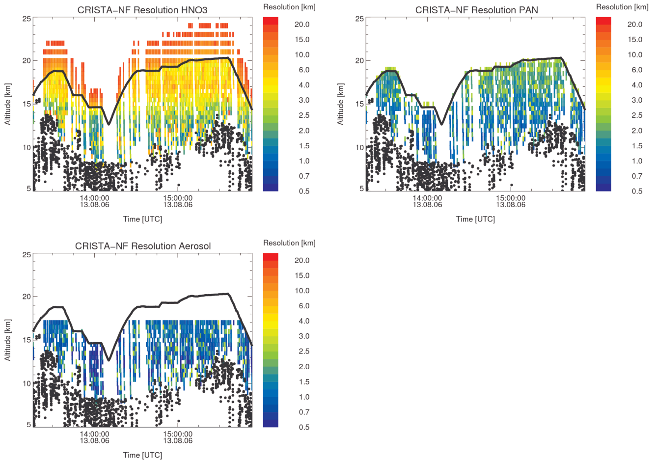
Fig. S2. CRISTA-NF resolution for all profiles during flight L5 for HNO 3 , Pan and aerosol extinction.
