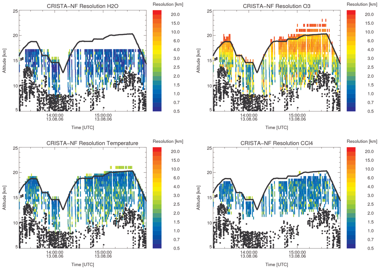
Fig. S1. CRISTA-NF resolution for all profiles during flight L5 for H 2 O, O 3 , temperature and CCl 4 .
