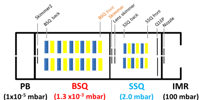
Figure 1. Schematic of the Tofwerk atmospheric pressure interface (API) showing where the IMR mounts on the API, the short segmented quadrupole (SSQ), the big segmented quadrupole (BSQ), and the primary beam (PB) region.
