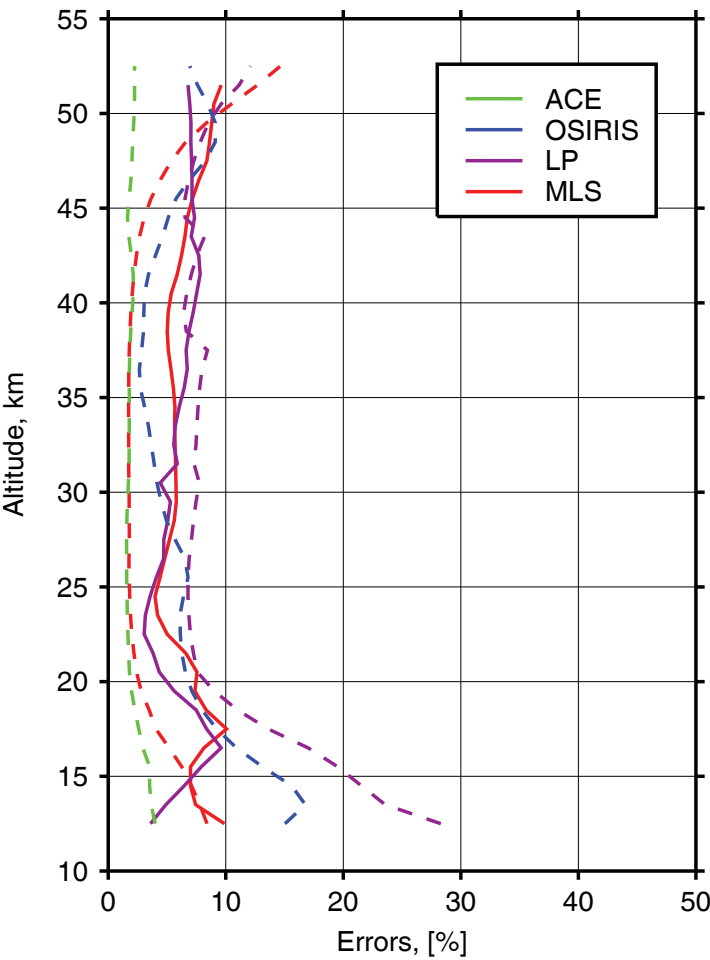
(a) Systematic and random errors, [%], mid-latitudes
