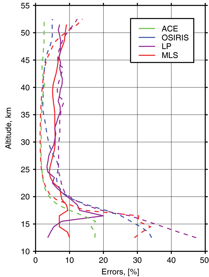
(b) Systematic and random errors, [%], tropics
