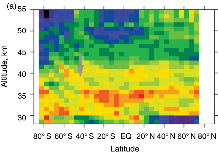
Differences OMPS-LP v2.5 - MLS v4, 10/23/2015
