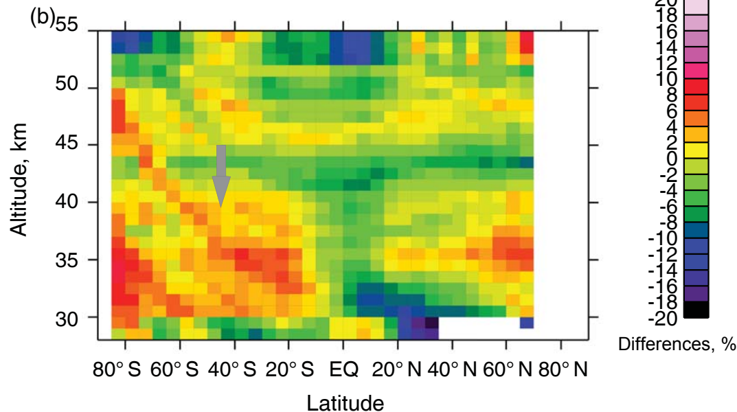
Differences OMPS-LP v2.5 - MLS v4, 11/05/2015
