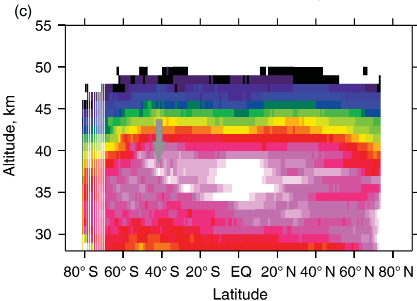
Measured radiances at 312 nm, 10/23/2015
