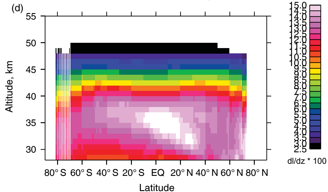
Calculated radiances at 312 nm, 10/23/2015
