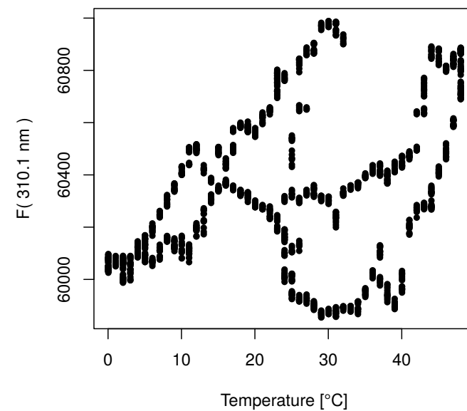
External lamp (dir) in ozone mode (Slit 2) at K&Z
