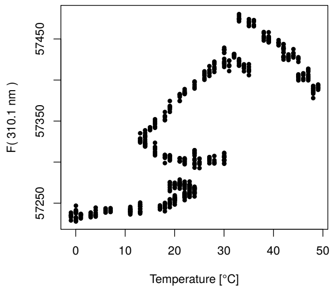
Internal lamp in ozone mode (Slit 2) at PTB1
