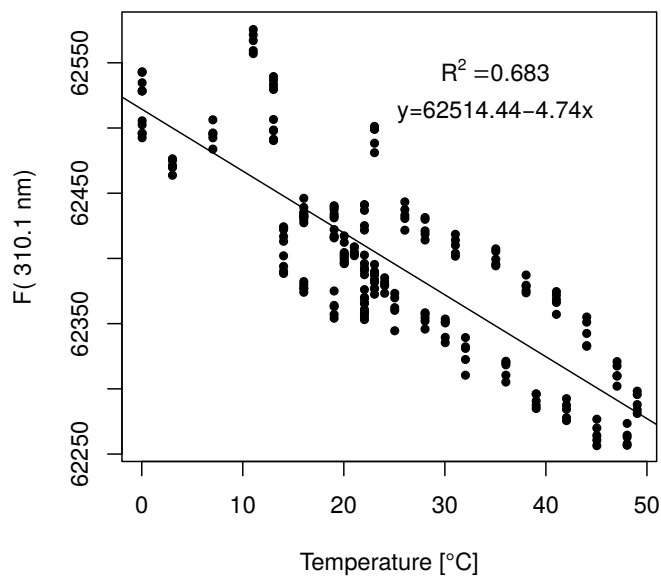
External lamp (dir) in ozone mode (Slit 2) at PTB1
