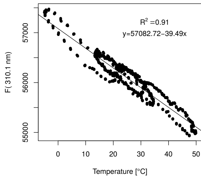
External lamp (dir) in ozone mode (Slit 2) at PTB2
