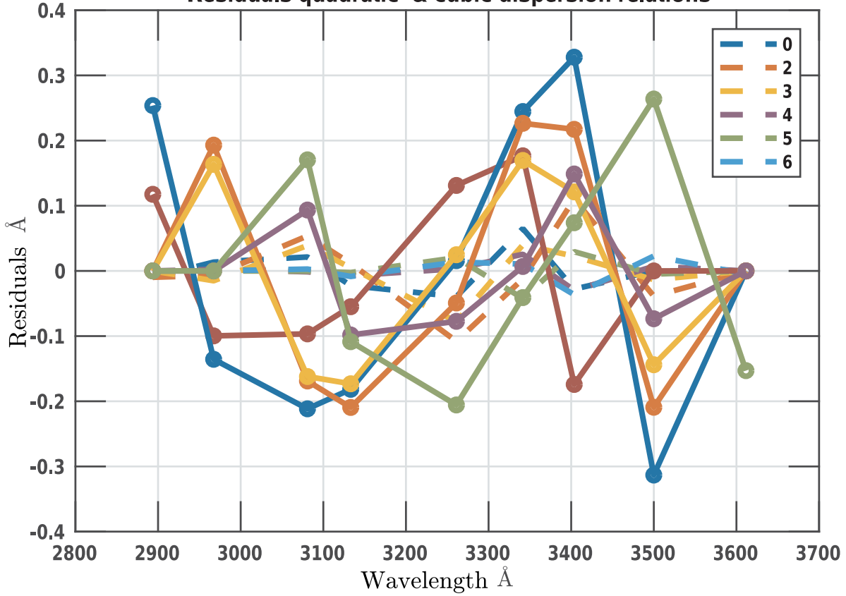
Residuals quadratic &amp; cubic dispersion relations
