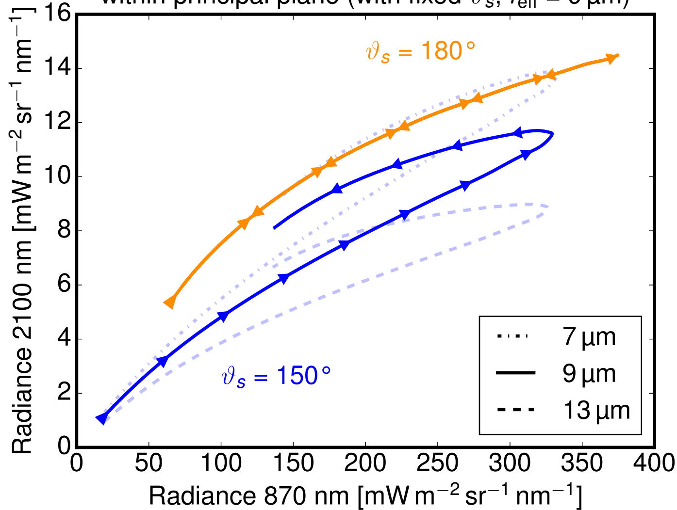
Spectral reflection for cloud surface tilting within principal plane (with fixed \vartheta_s , r_{\text{eff}} = 9 \mu\text{m} )
