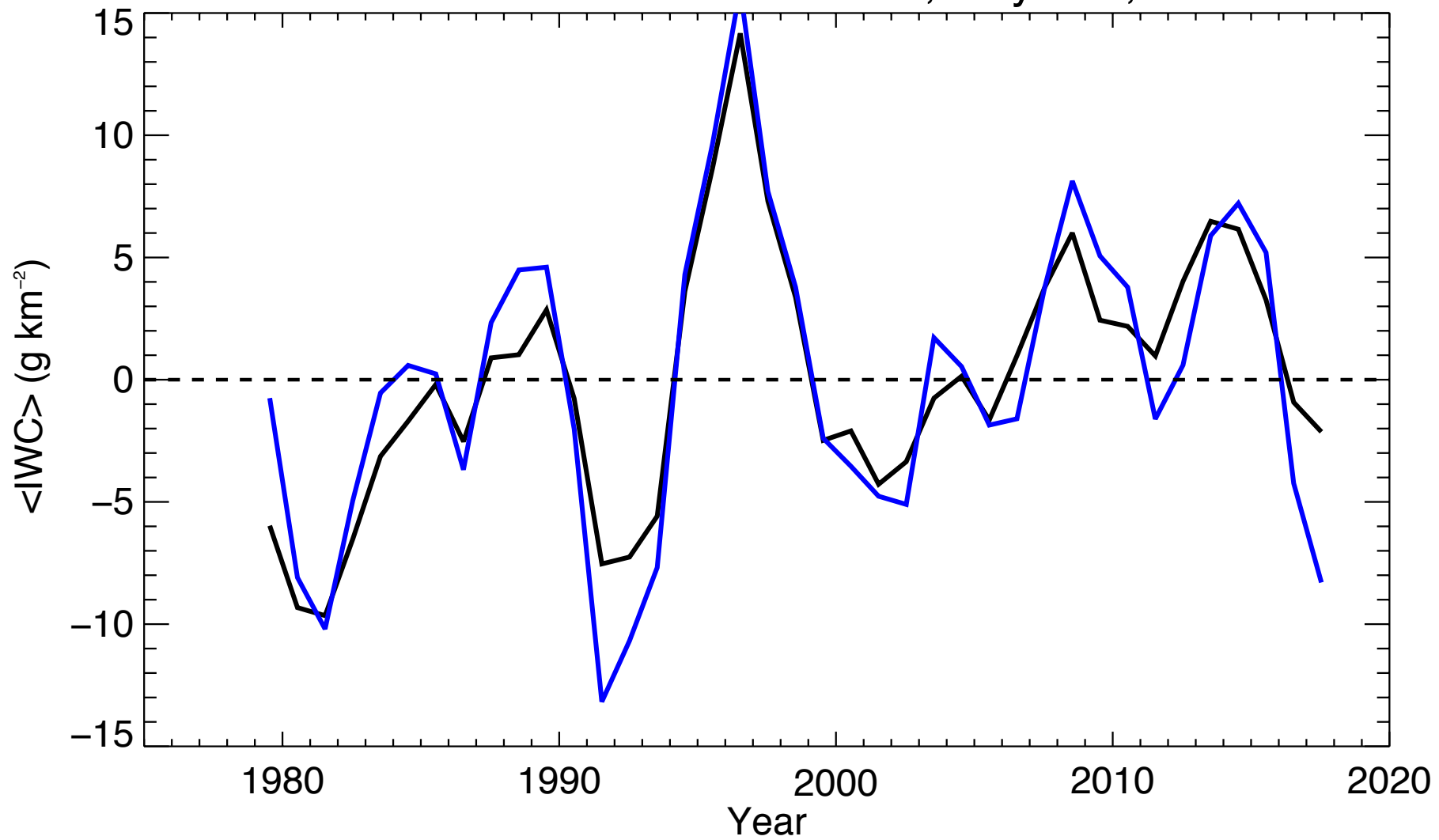
SBUV IWC residual, July ave, NH
