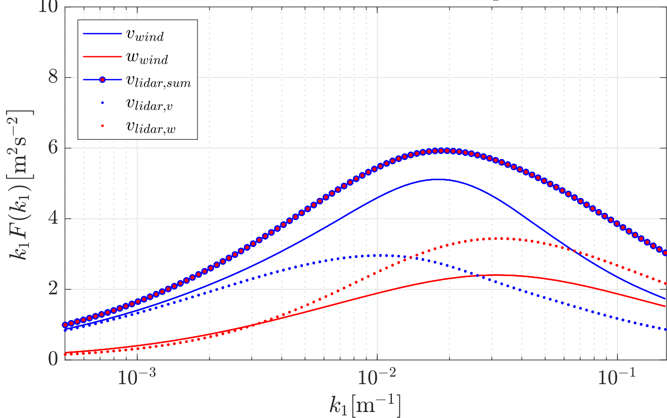
(b) \times 10^{-2} Cross-contamination for lateral separation
