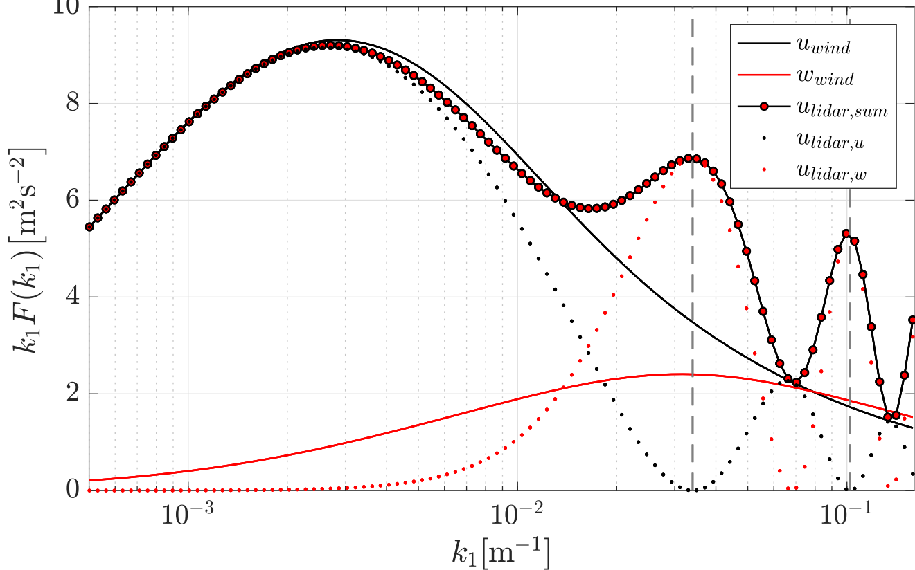
(a) \times 10^{-2} Cross-contamination for longitudinal separation
