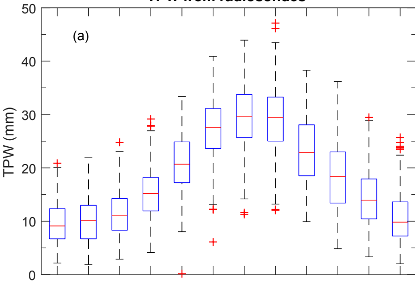
TPW from radiosondes
