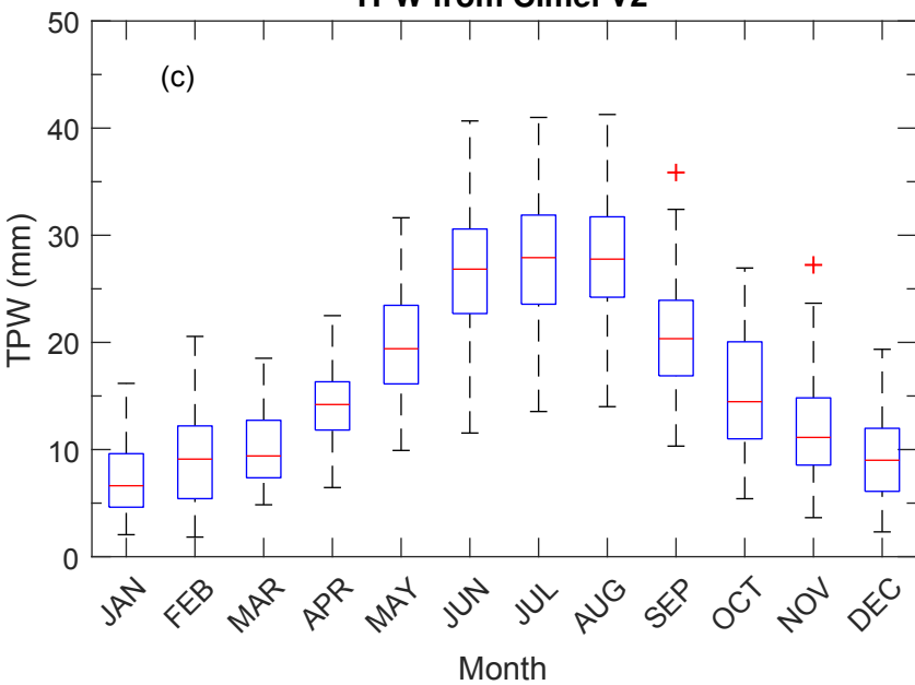
TPW from Cimel V2
