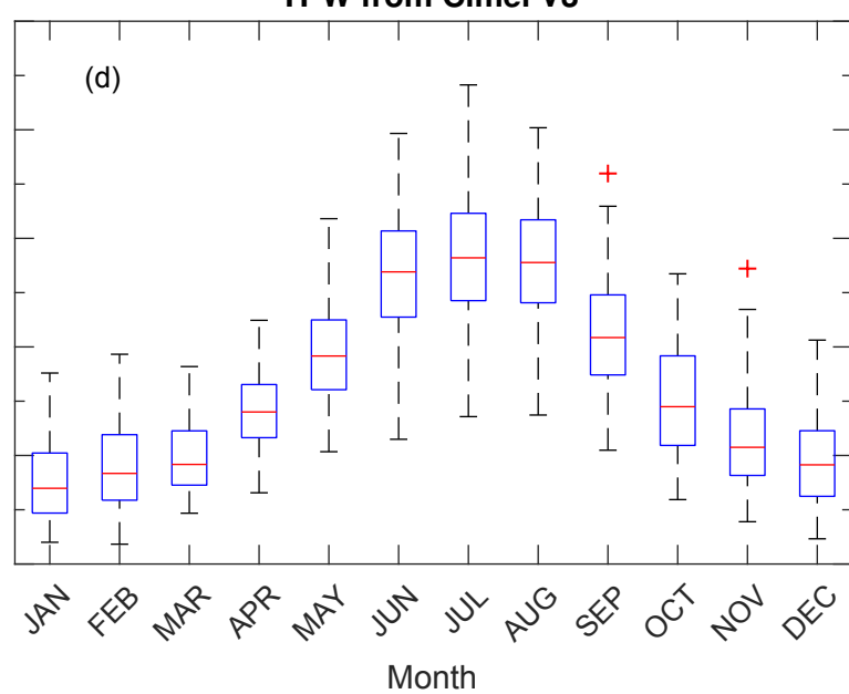
TPW from Cimel V3
