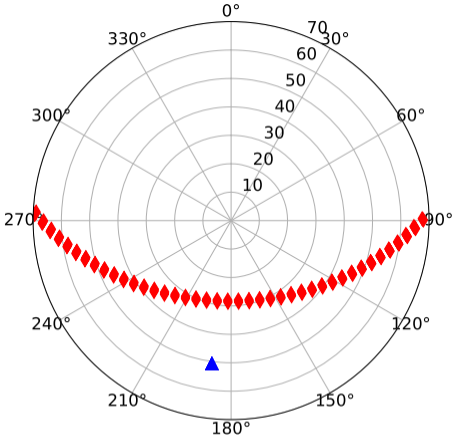
(a) SEVIRI
