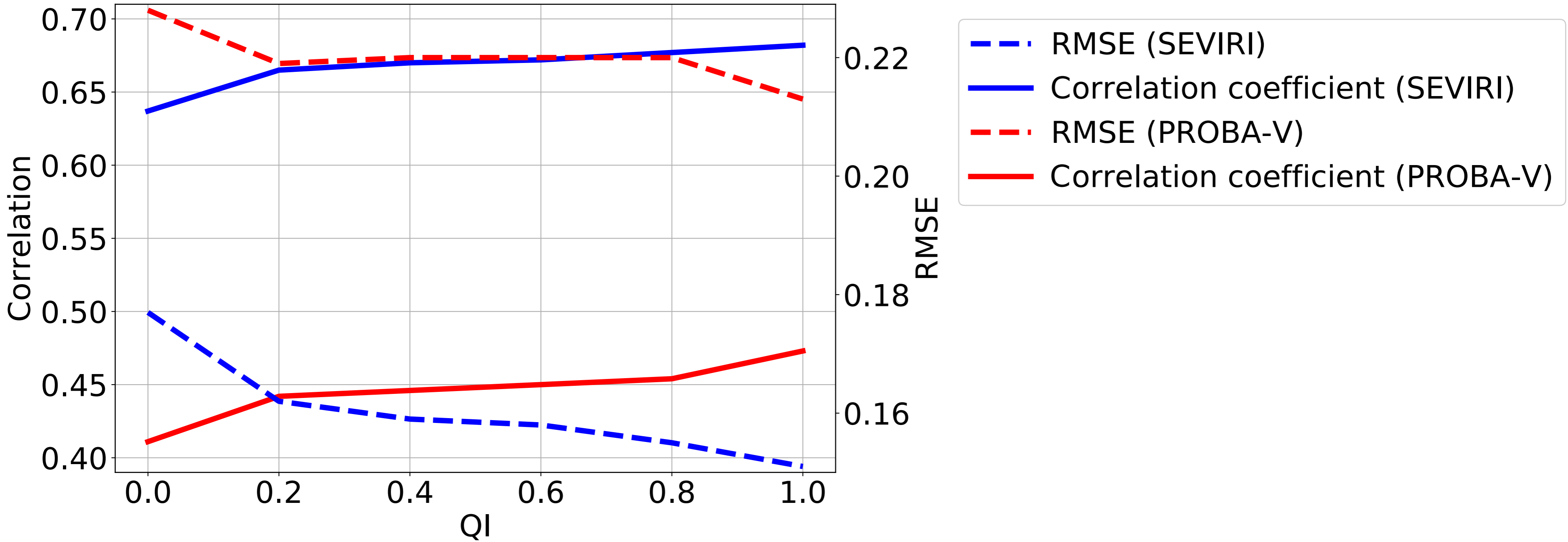
CISAR vs. AERONET AOT
