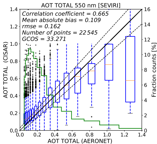
(a) SEVIRI
