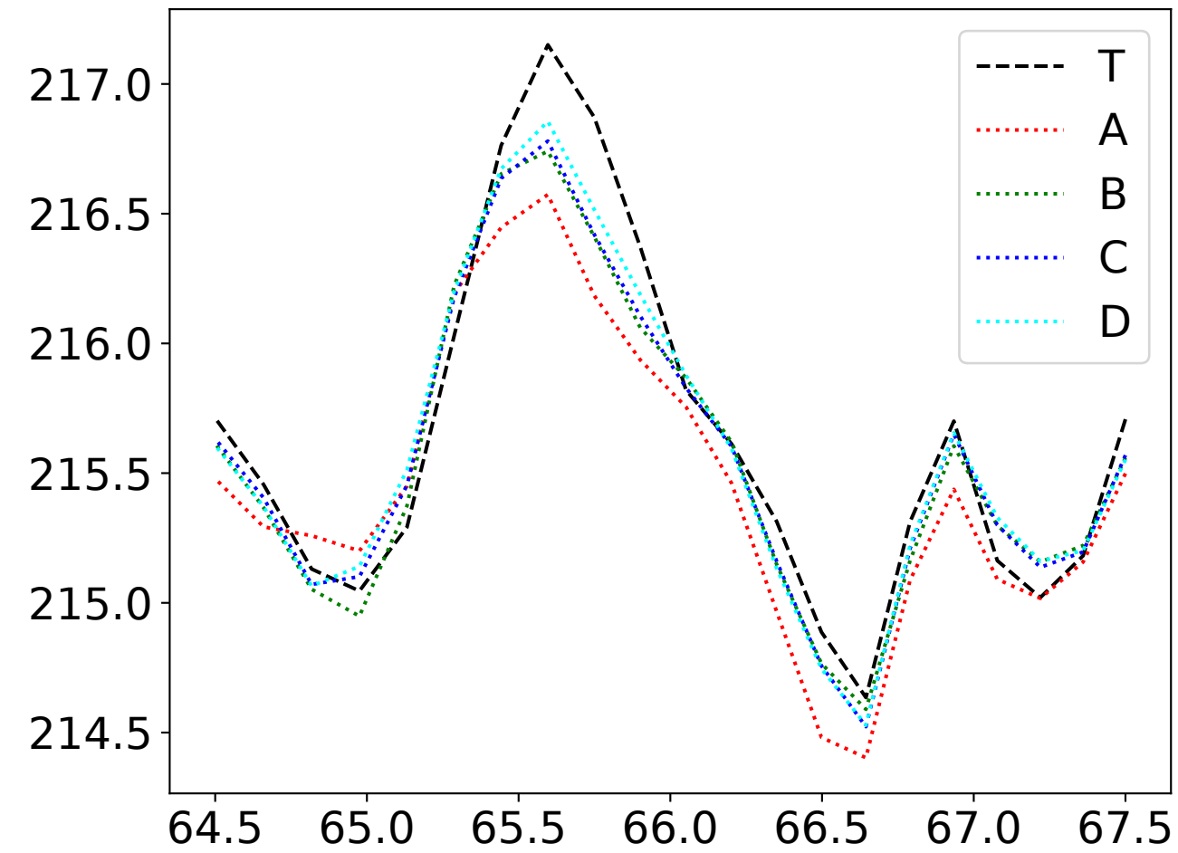
H = 13 km
