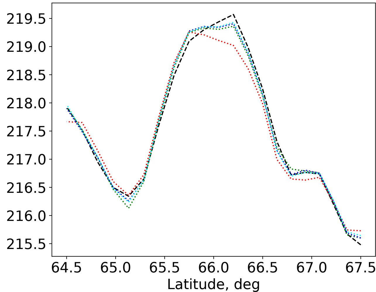
H = 12 km
