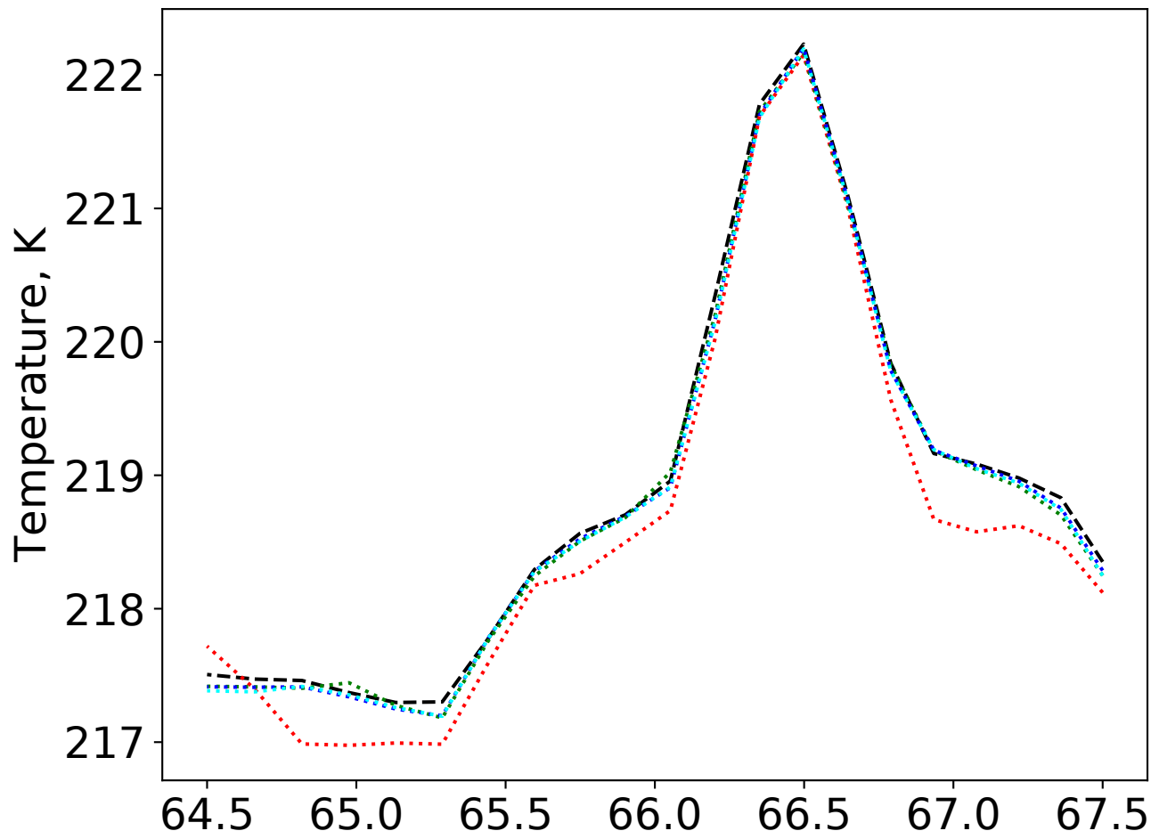
H = 10.5 km
